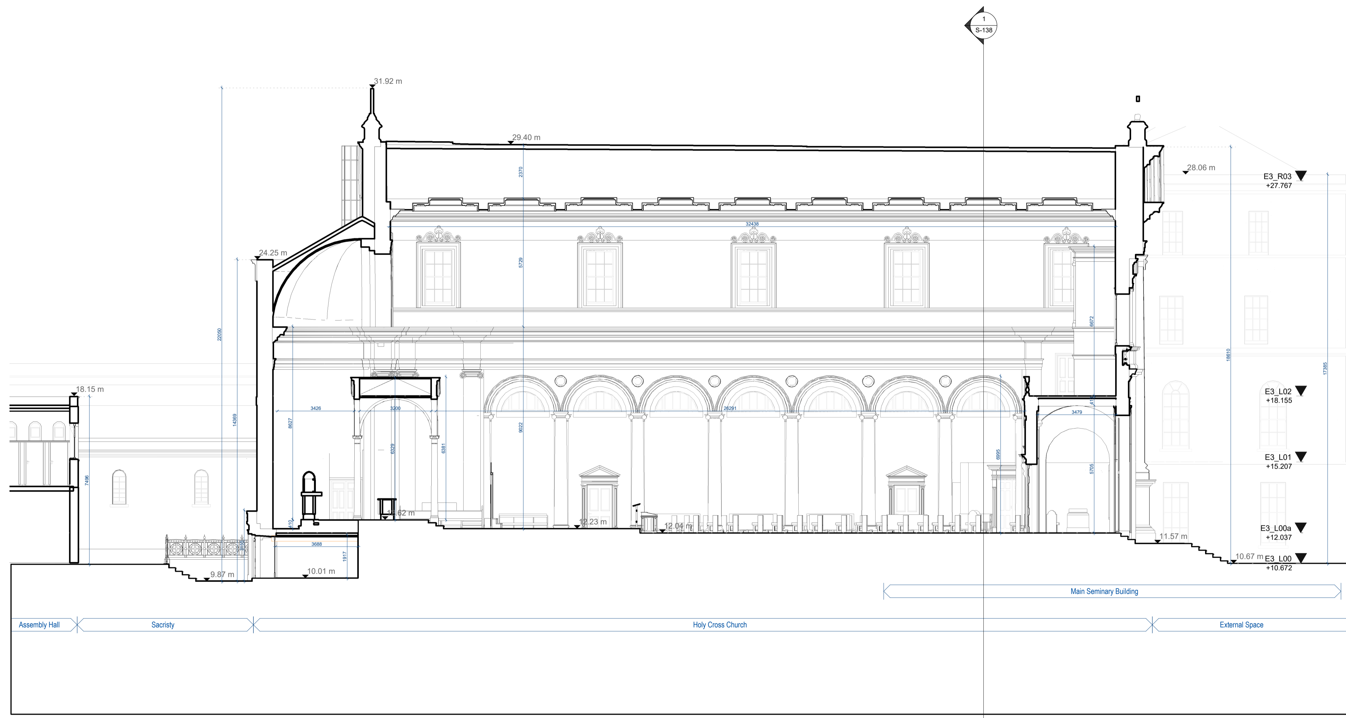
1 Section-AA-Survey Scale - 1:100
